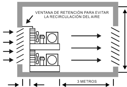
Corte Vertical
